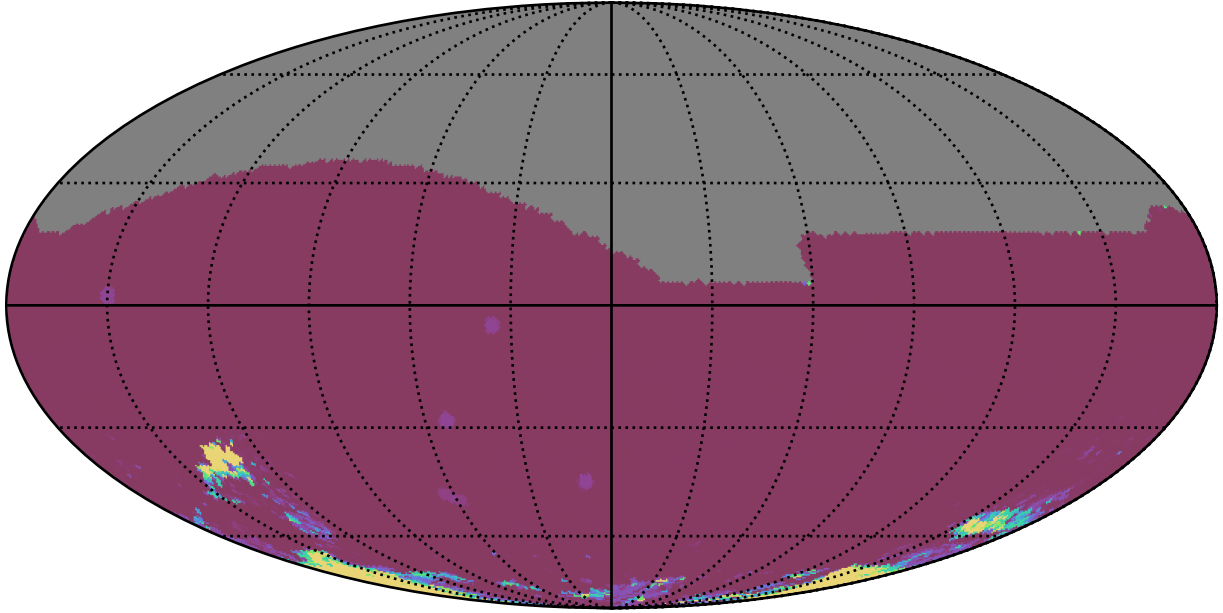
telescope_jerk_v3.5_10yrs All sky iz bands: 75th Percentile Intranight Timespan
