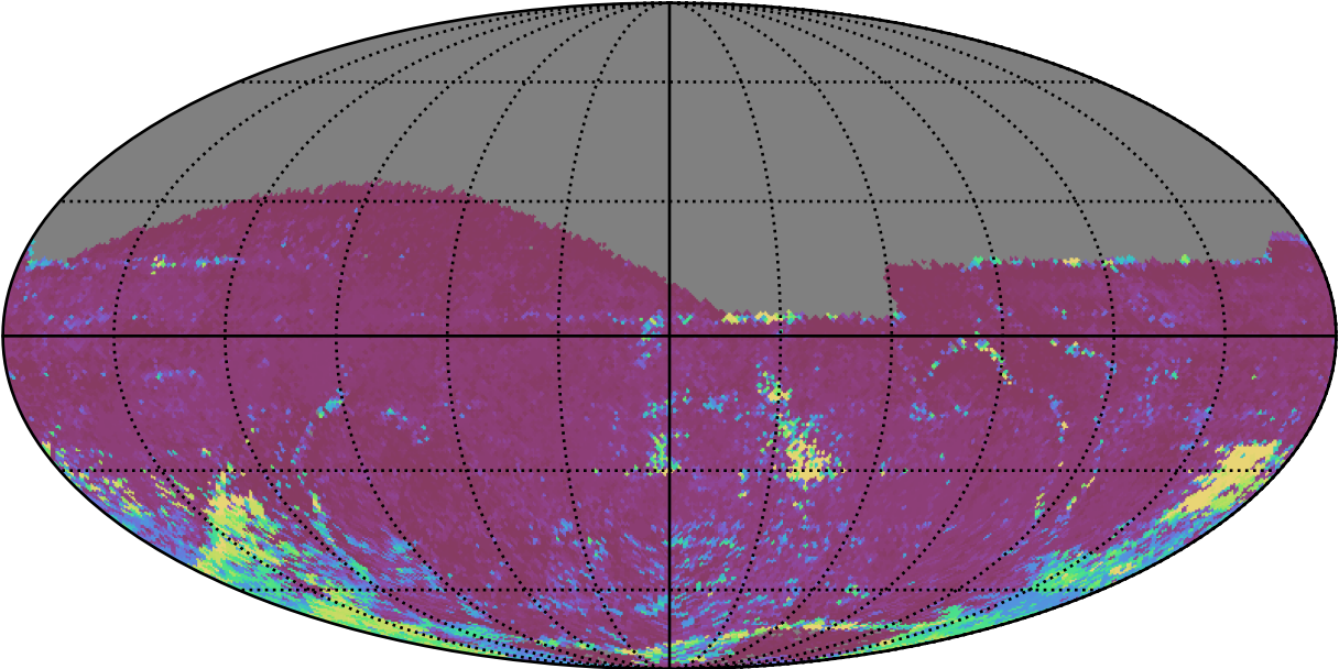
telescope_jerk_v3.5_10yrs All sky i band: 75th Percentile Intranight Timespan
