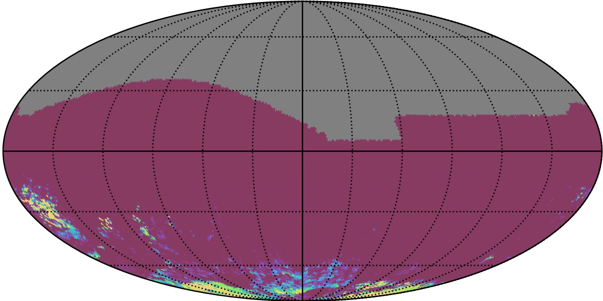
telescope_jerk_v3.5_10yrs All sky gr bands: 75th Percentile Intranight Timespan
