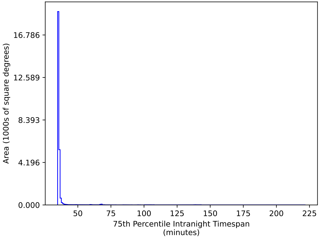
telescope_jerk_v3.5_10yrs All sky gr bands: 75th Percentile Intranight Timespan
