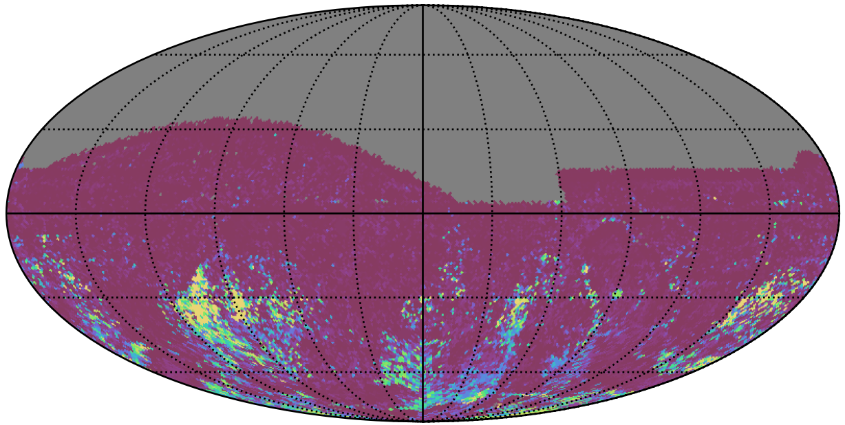
telescope_jerk_v3.5_10yrs All sky g band: 75th Percentile Intranight Timespan
