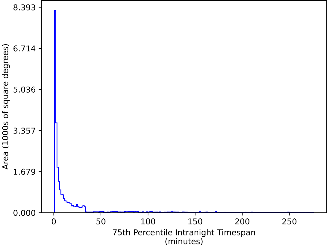
telescope_jerk_v3.5_10yrs All sky g band: 75th Percentile Intranight Timespan
