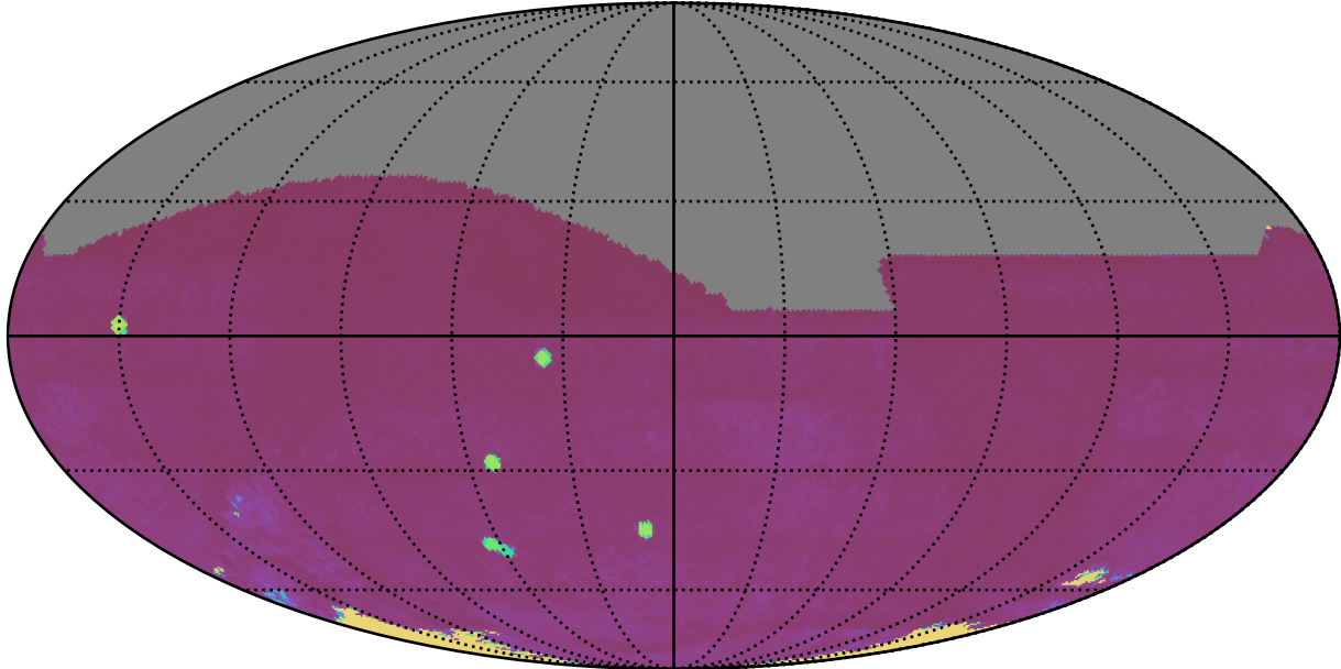
telescope_jerk_v3.5_10yrs All sky all bands: 75th Percentile Intranight Timespan
