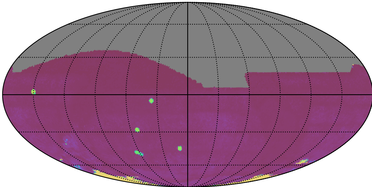
telescope_jerk_v3.5_10yrs All sky: 75th Percentile Intranight Timespan
