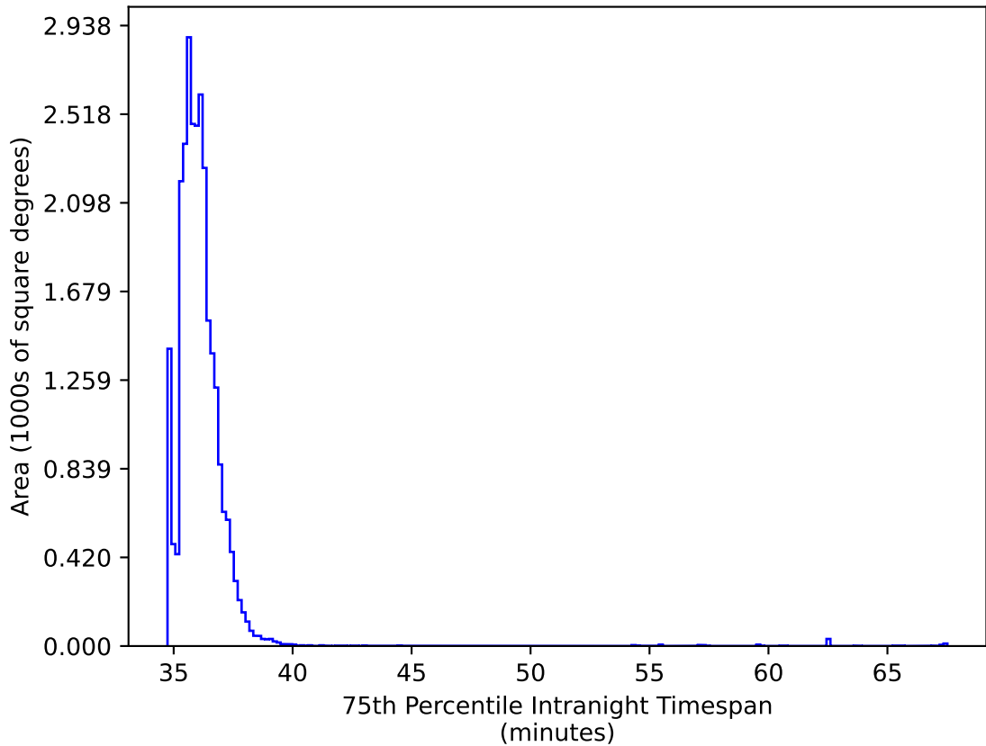
telescope_jerk_v3.5_10yrs All sky: 75th Percentile Intranight Timespan
