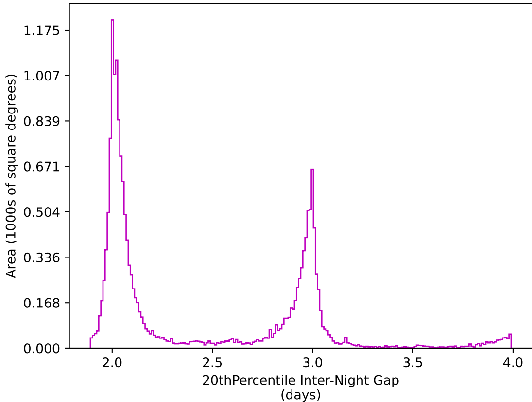
telescope_jerk_v3.5_10yrs WFD z band: 20thPercentile Inter-Night Gap
