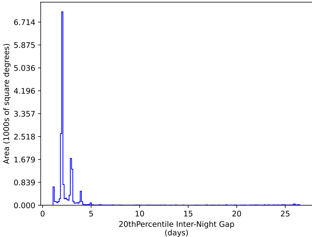
telescope_jerk_v3.5_10yrs WFD y band: 20thPercentile Inter-Night Gap
