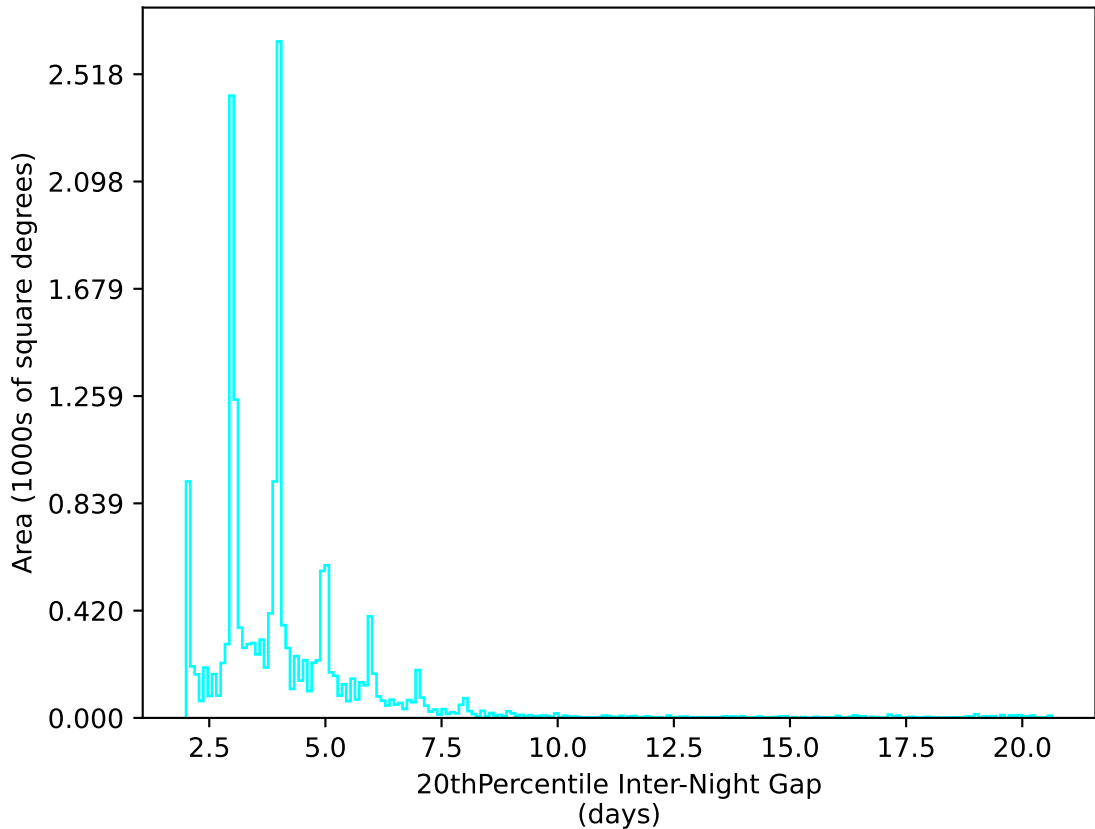
telescope_jerk_v3.5_10yrs WFD u band: 20thPercentile Inter-Night Gap
