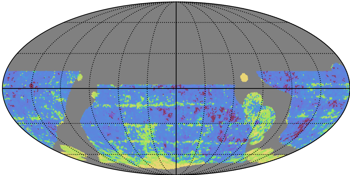
telescope_jerk_v3.5_10yrs WFD r band: 20thPercentile Inter-Night Gap
