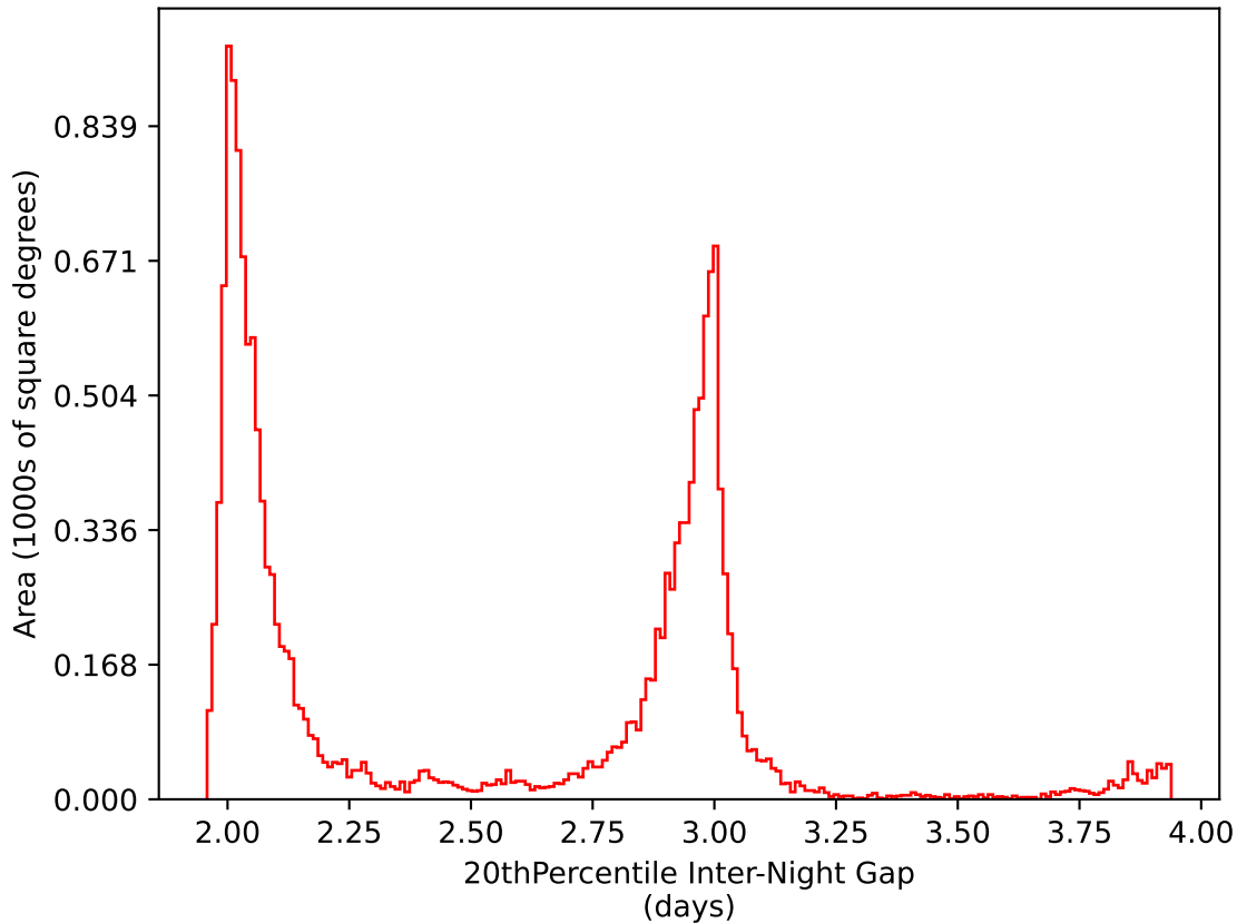
telescope_jerk_v3.5_10yrs WFD i band: 20thPercentile Inter-Night Gap
