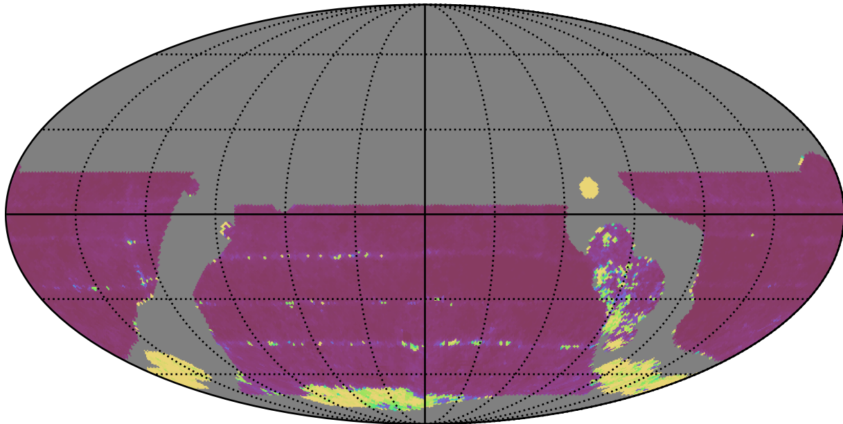
telescope_jerk_v3.5_10yrs WFD all bands: 20thPercentile Inter-Night Gap
