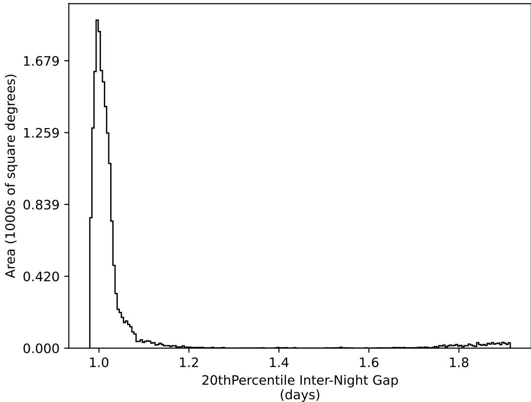
telescope_jerk_v3.5_10yrs WFD all bands: 20thPercentile Inter-Night Gap
