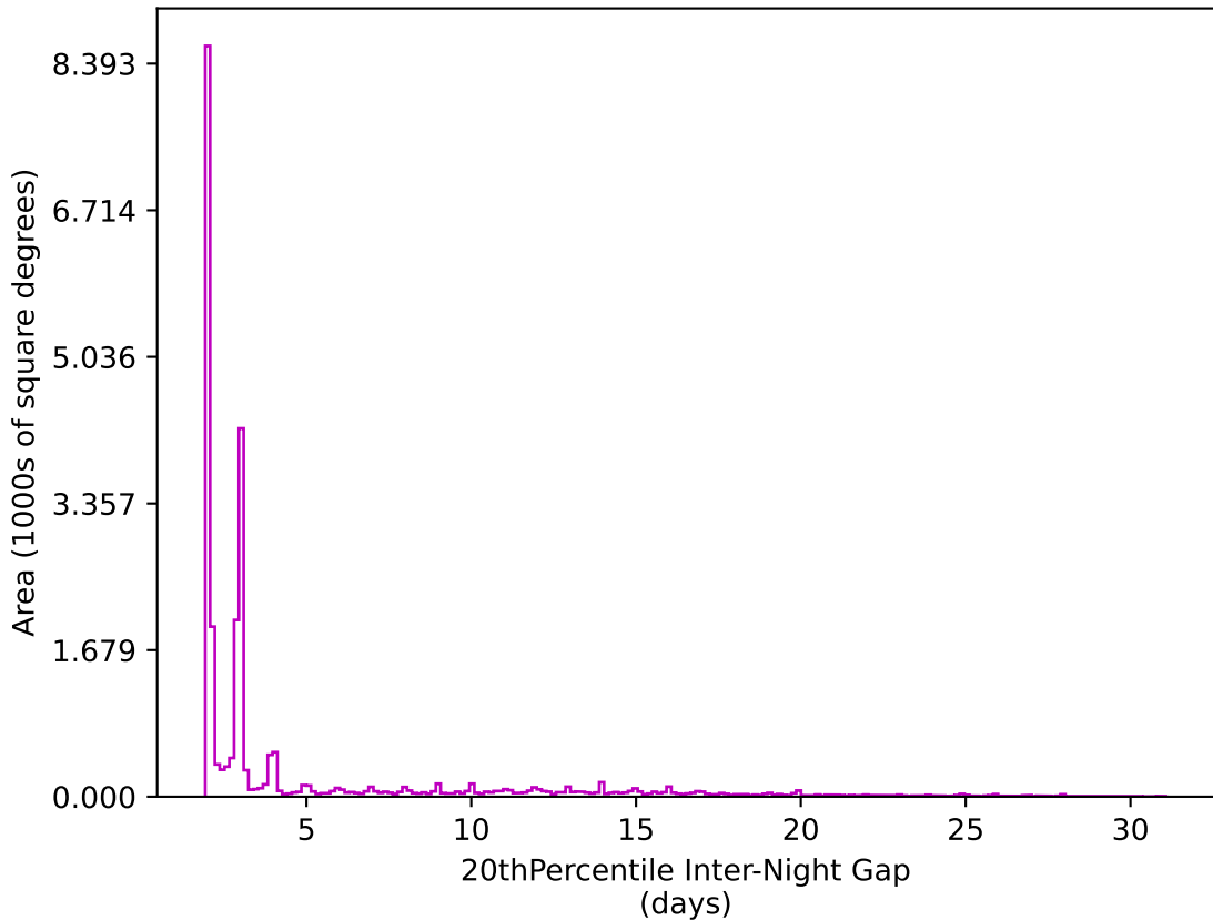
telescope_jerk_v3.5_10yrs All sky z band: 20thPercentile Inter-Night Gap
