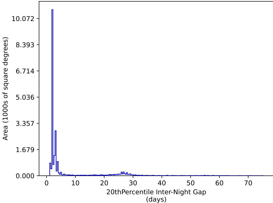
telescope_jerk_v3.5_10yrs All sky y band: 20thPercentile Inter-Night Gap
