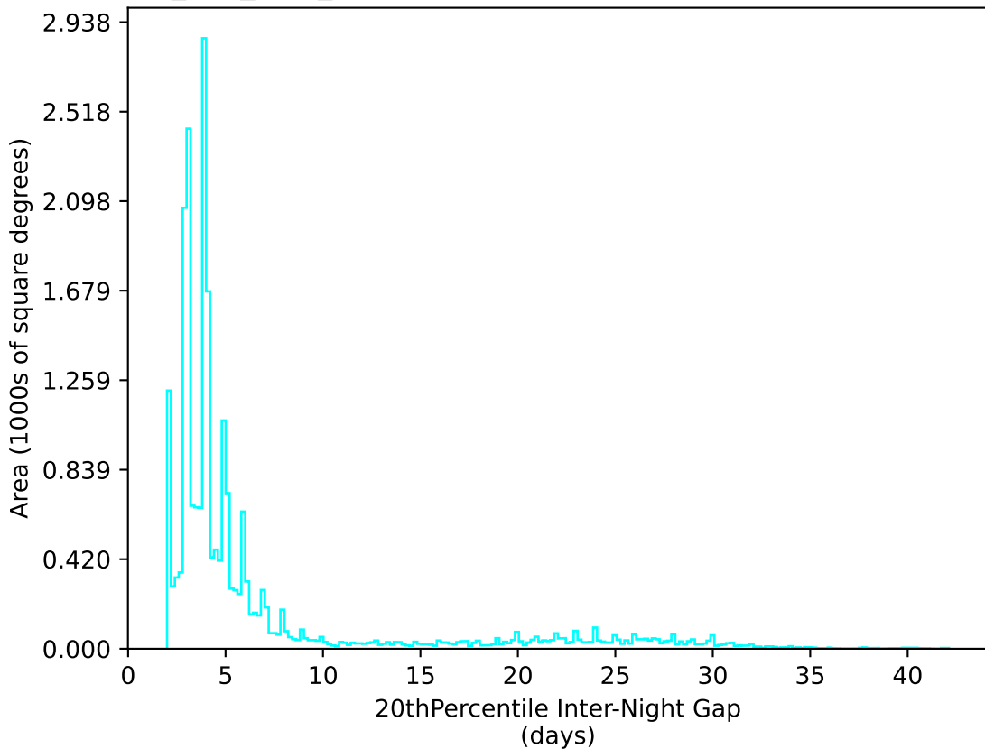
telescope_jerk_v3.5_10yrs All sky u band: 20thPercentile Inter-Night Gap
