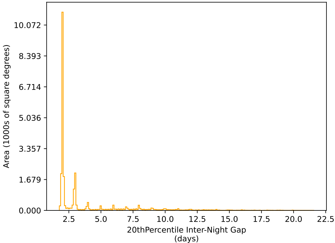
telescope_jerk_v3.5_10yrs All sky r band: 20thPercentile Inter-Night Gap
