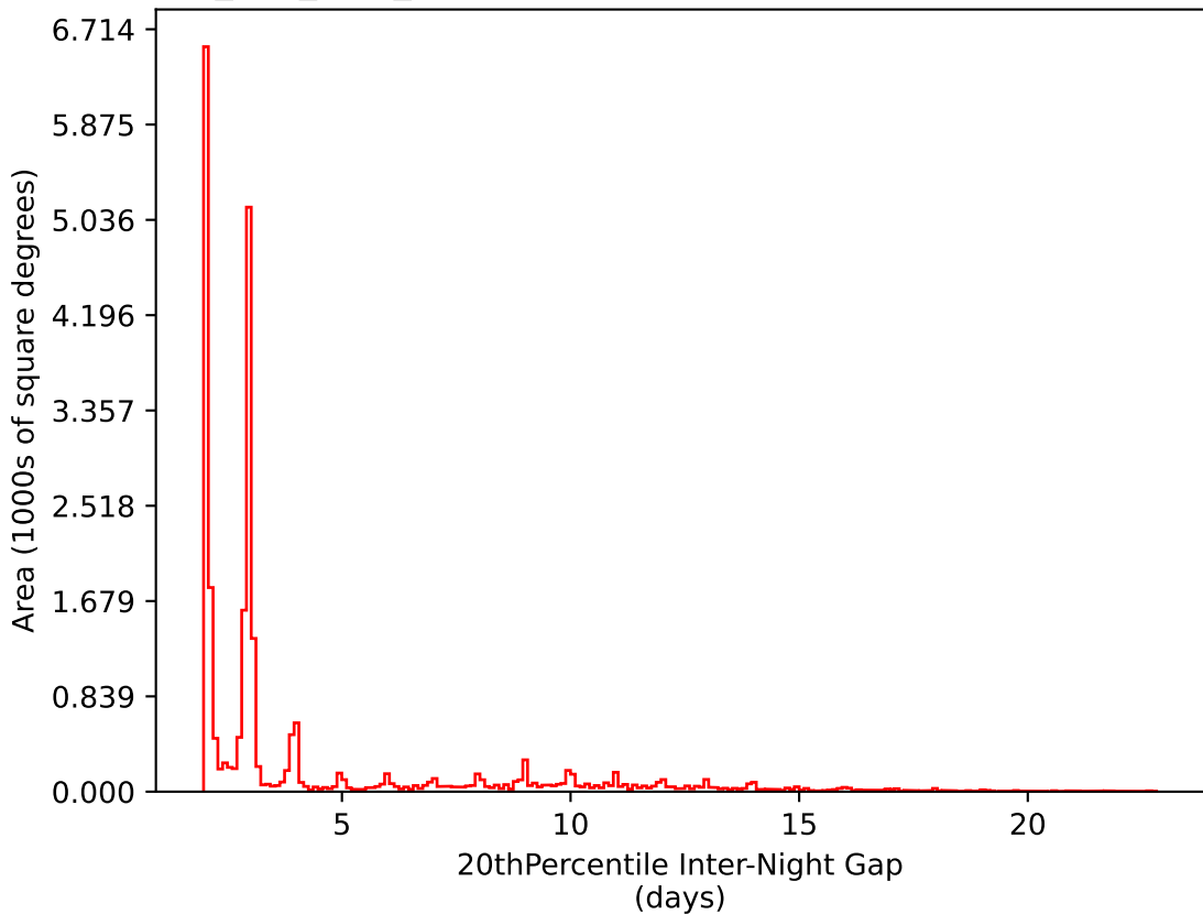
telescope_jerk_v3.5_10yrs All sky i band: 20thPercentile Inter-Night Gap
