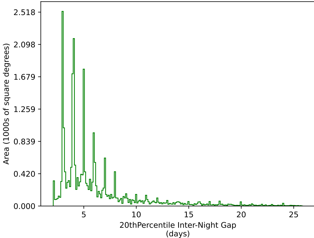
telescope_jerk_v3.5_10yrs All sky g band: 20thPercentile Inter-Night Gap
