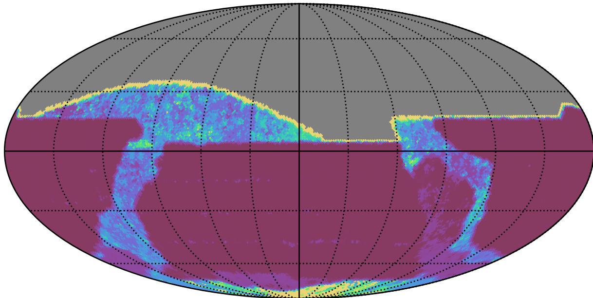
telescope_jerk_v3.5_10yrs All sky all bands: 20thPercentile Inter-Night Gap
