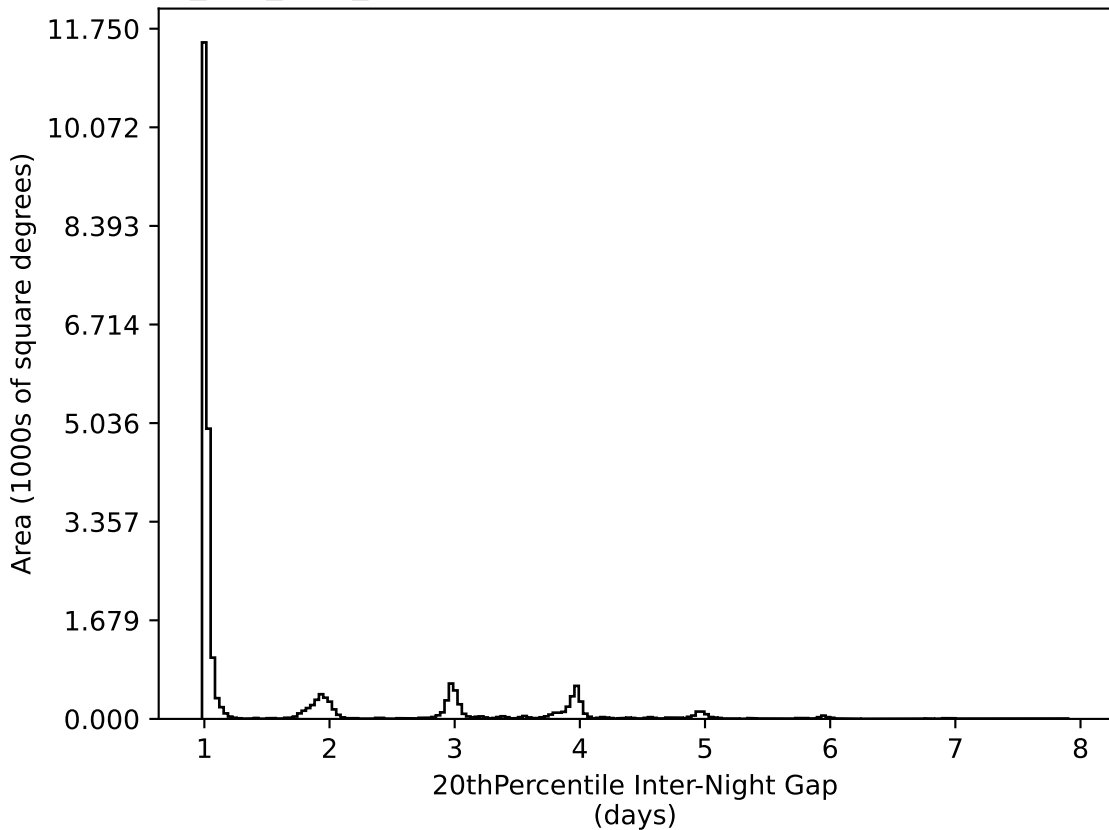
telescope_jerk_v3.5_10yrs All sky all bands: 20thPercentile Inter-Night Gap
