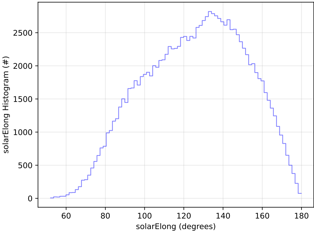
start_date_do90v3.4_10yrs WFD u band: solarElong Histogram
