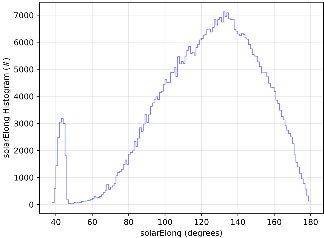
start_date_do90v3.4_10yrs WFD r band: solarElong Histogram
