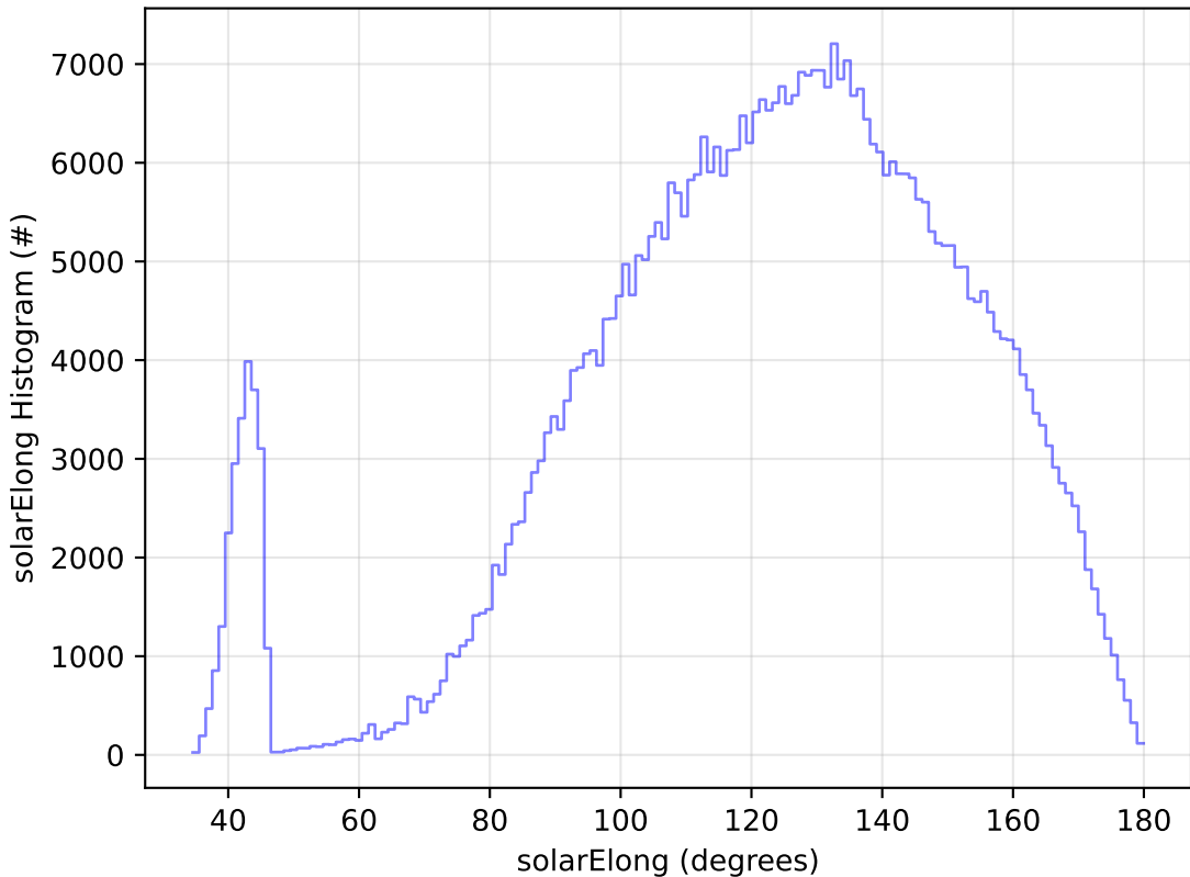
start_date_do90v3.4_10yrs WFD i band: solarElong Histogram
