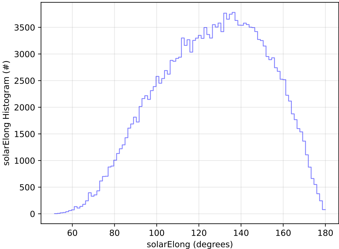
start_date_do90v3.4_10yrs WFD g band: solarElong Histogram
