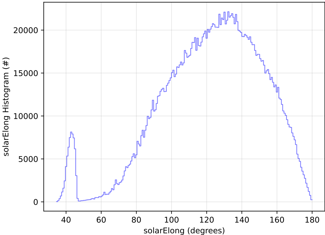
start_date_do90v3.4_10yrs WFD all bands: solarElong Histogram
