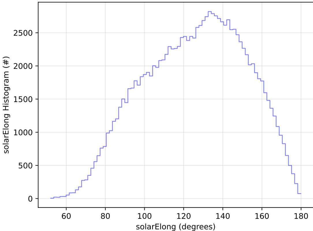
start_date_do90v3.4_10yrs All sky u band: solarElong Histogram
