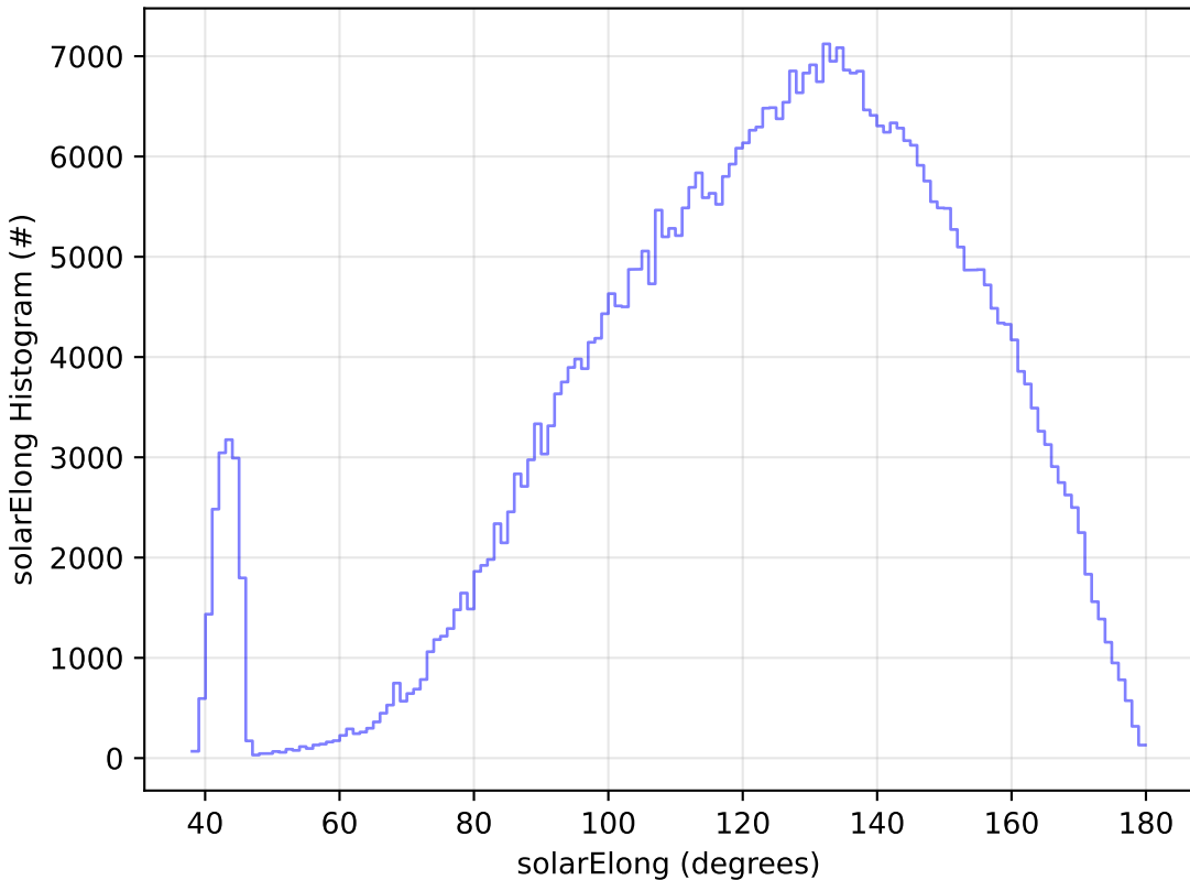
start_date_do90v3.4_10yrs All sky r band: solarElong Histogram
