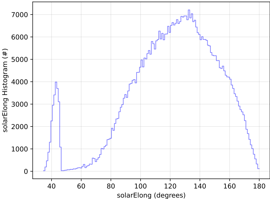
start_date_do90v3.4_10yrs All sky i band: solarElong Histogram
