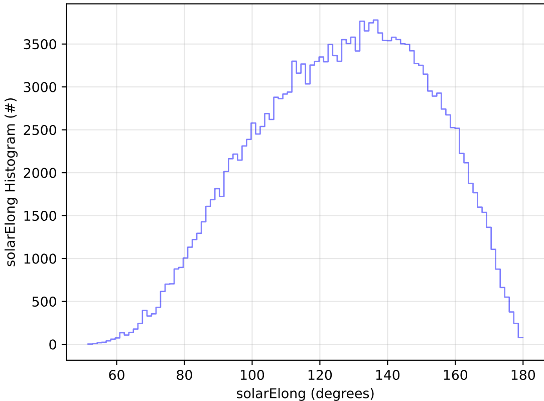
start_date_do90v3.4_10yrs All sky g band: solarElong Histogram
