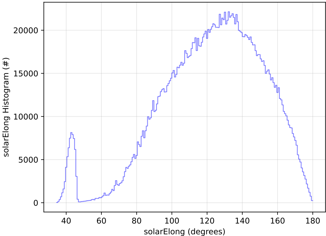
start_date_do90v3.4_10yrs All sky all bands: solarElong Histogram
