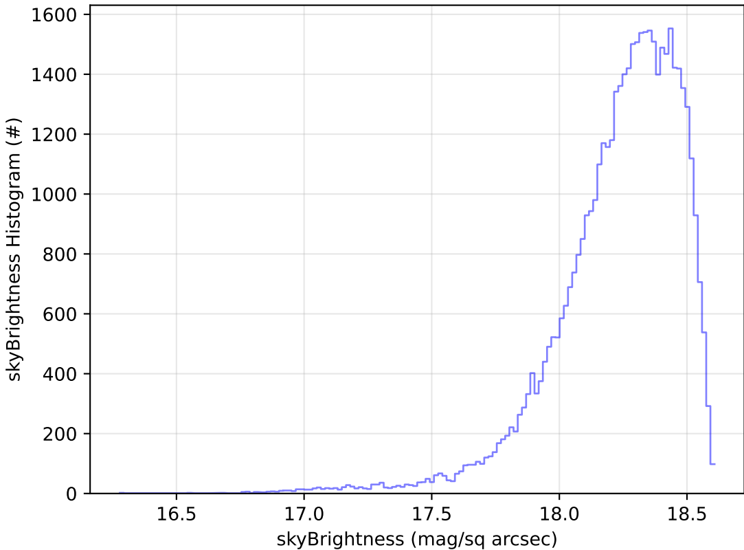
start_date_do90v3.4_10yrs Yr 1 y band: skyBrightness Histogram
