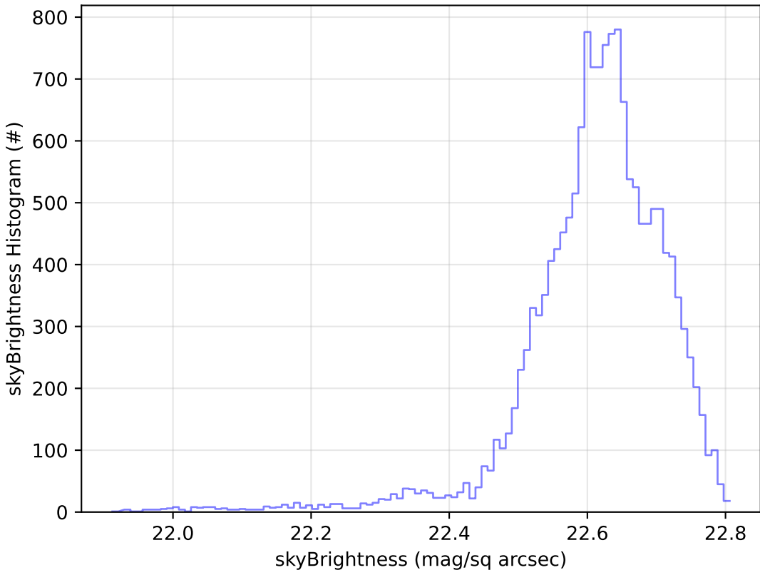
start_date_do90v3.4_10yrs Yr 1 u band: skyBrightness Histogram
