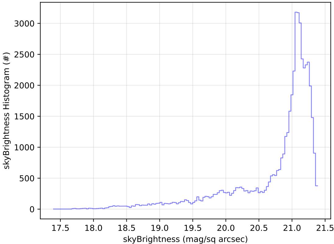
start_date_do90v3.4_10yrs Yr 1 r band: skyBrightness Histogram
