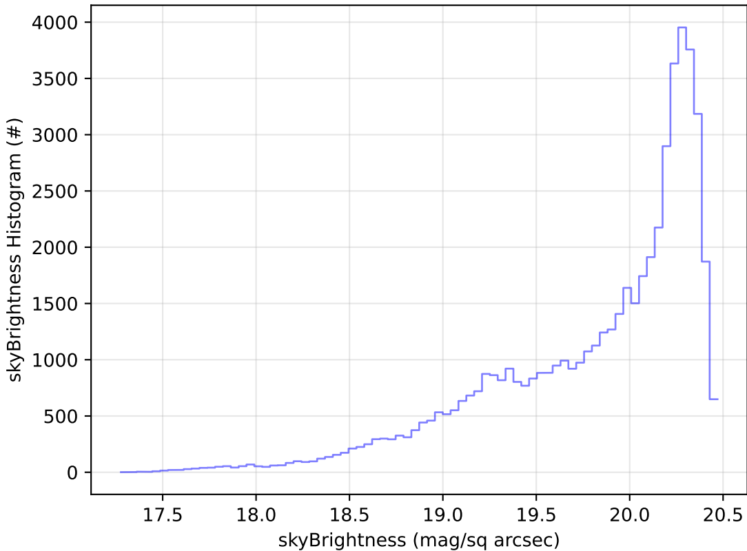
start_date_do90v3.4_10yrs Yr 1 i band: skyBrightness Histogram
