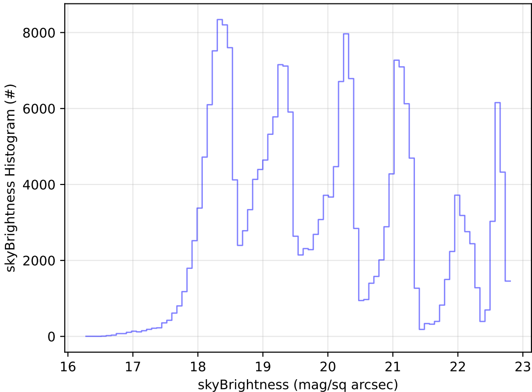
start_date_do90v3.4_10yrs Yr 1 all bands: skyBrightness Histogram
