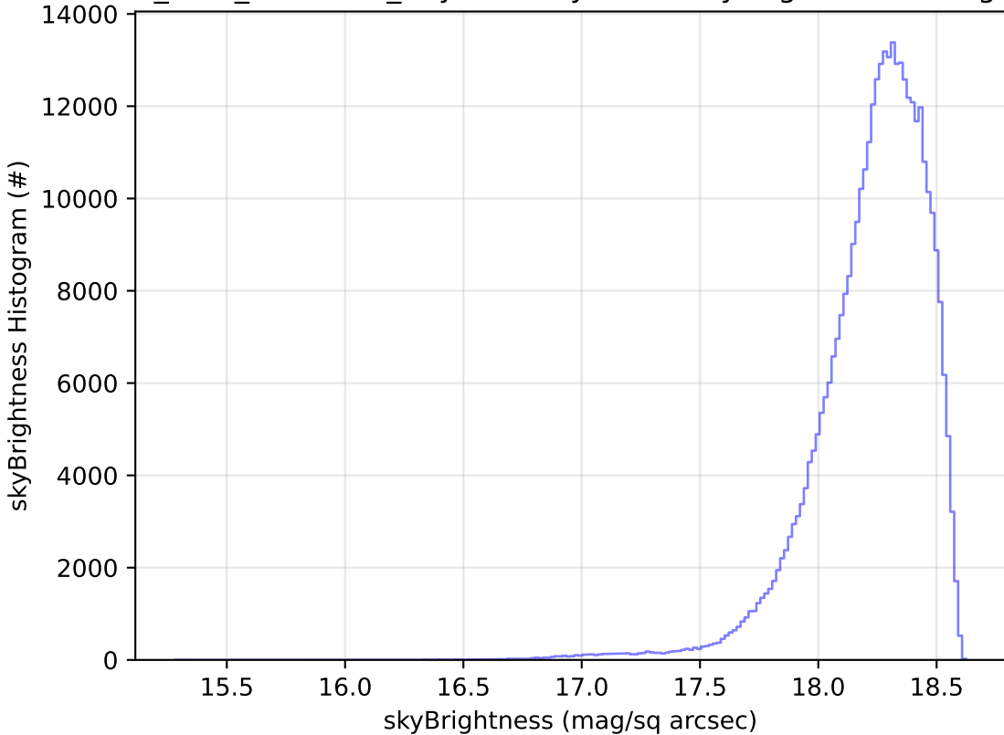
start_date_do90v3.4_10yrs WFD y band: skyBrightness Histogram
