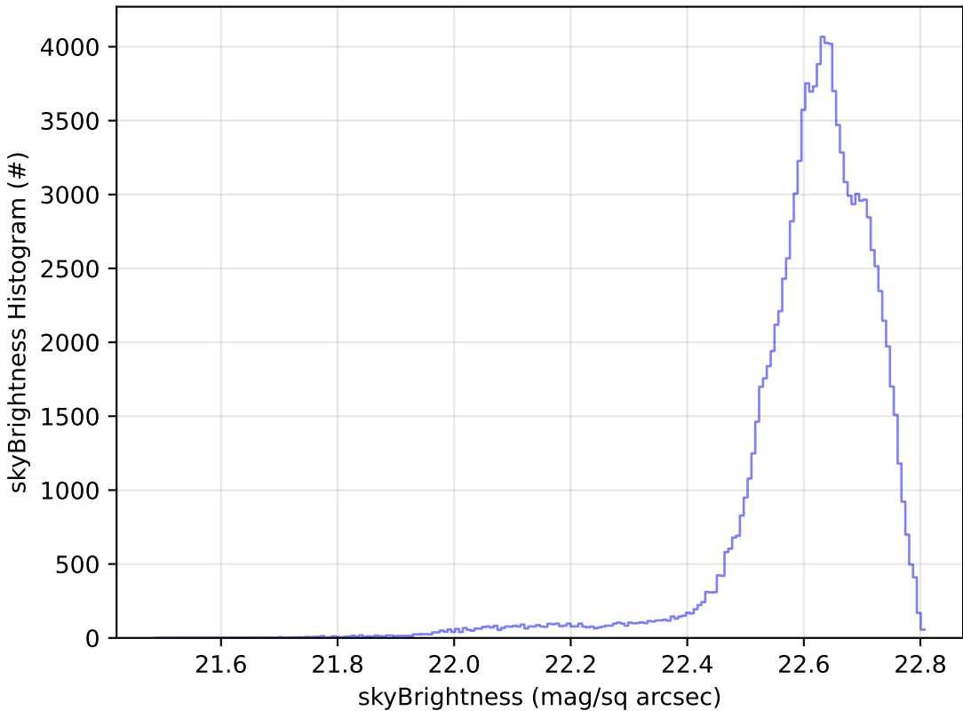
start_date_do90v3.4_10yrs WFD u band: skyBrightness Histogram
