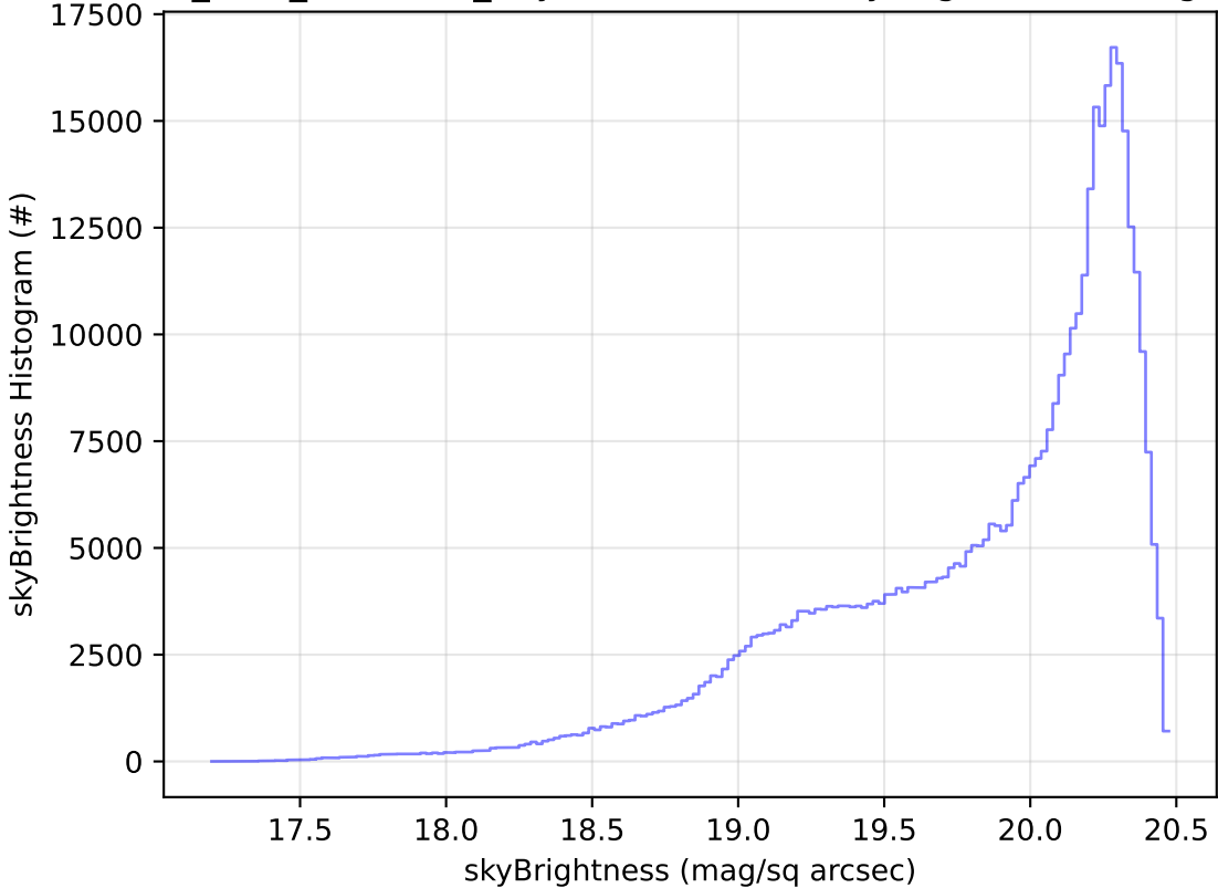
start_date_do90v3.4_10yrs WFD i band: skyBrightness Histogram
