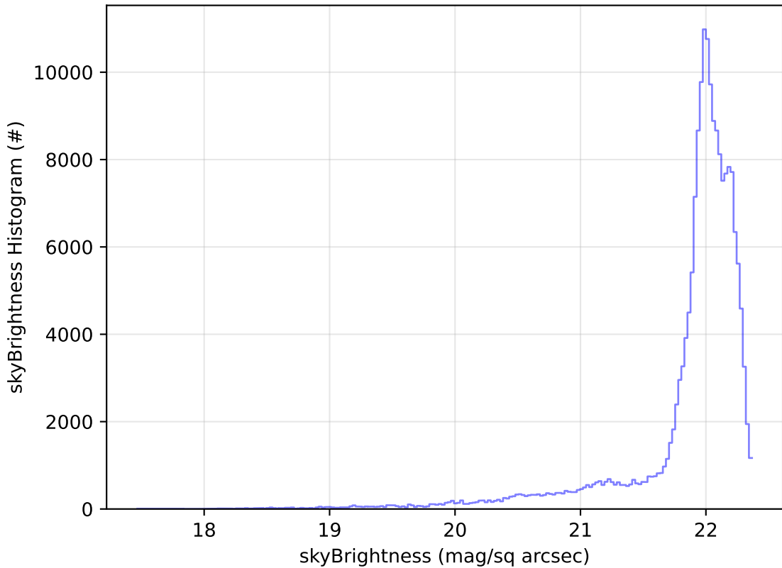
start_date_do90v3.4_10yrs WFD g band: skyBrightness Histogram
