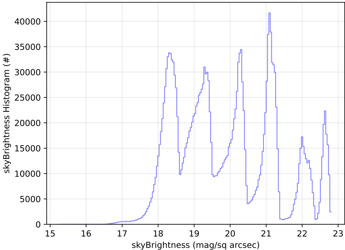
start_date_do90v3.4_10yrs WFD all bands: skyBrightness Histogram
