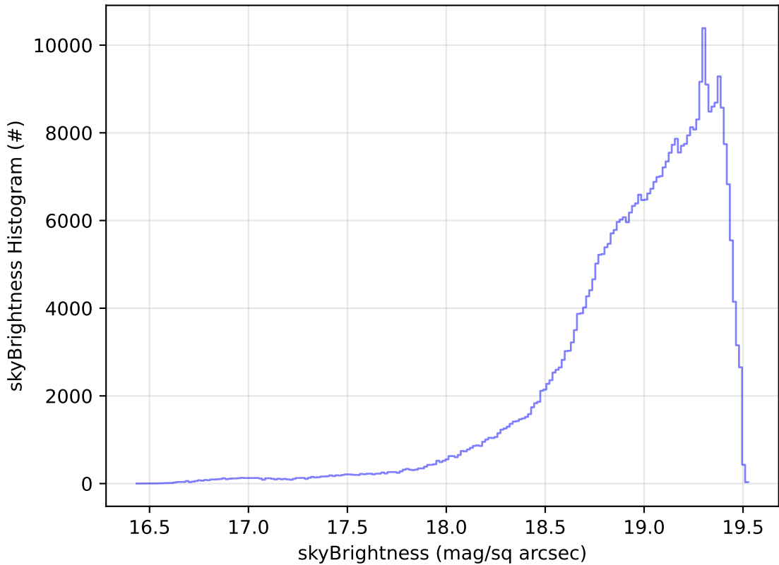
start_date_do90v3.4_10yrs All sky z band: skyBrightness Histogram
