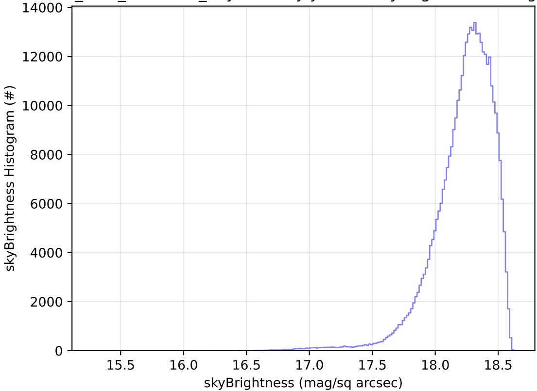
start_date_do90v3.4_10yrs All sky y band: skyBrightness Histogram
