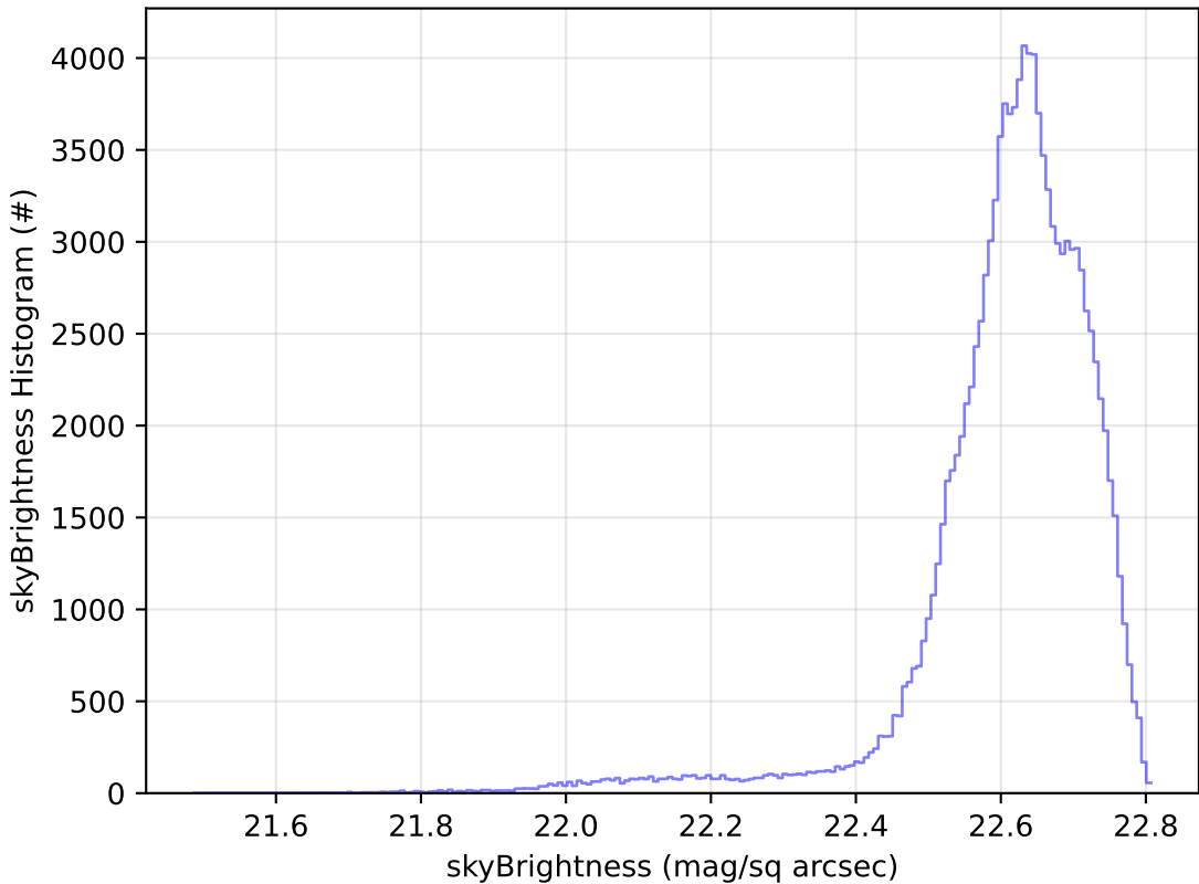
start_date_do90v3.4_10yrs All sky u band: skyBrightness Histogram
