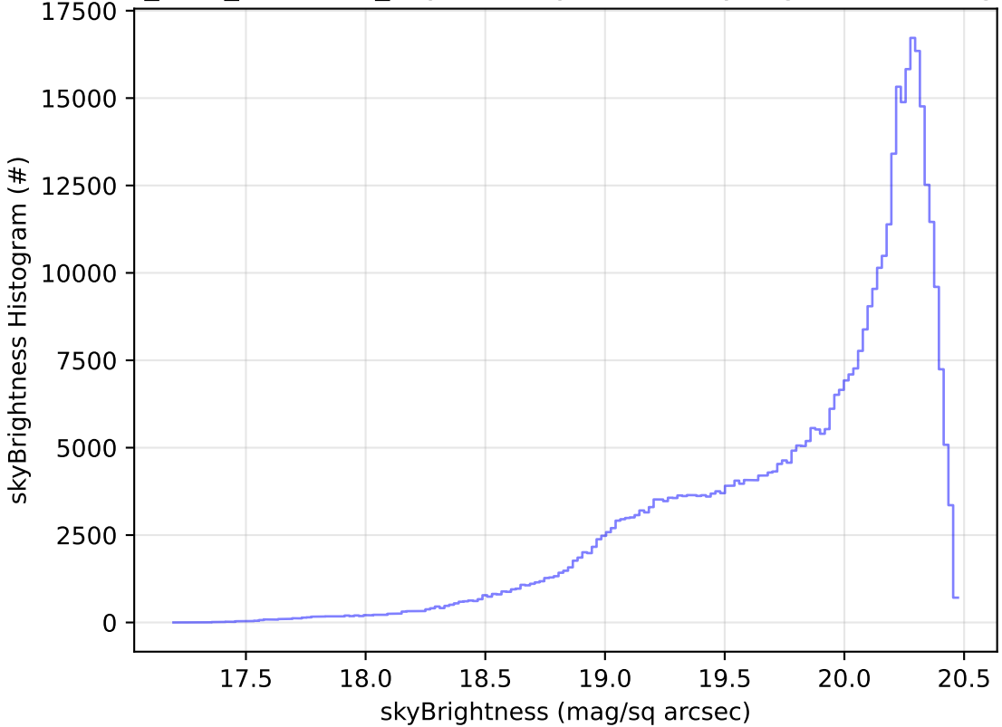
start_date_do90v3.4_10yrs All sky i band: skyBrightness Histogram
