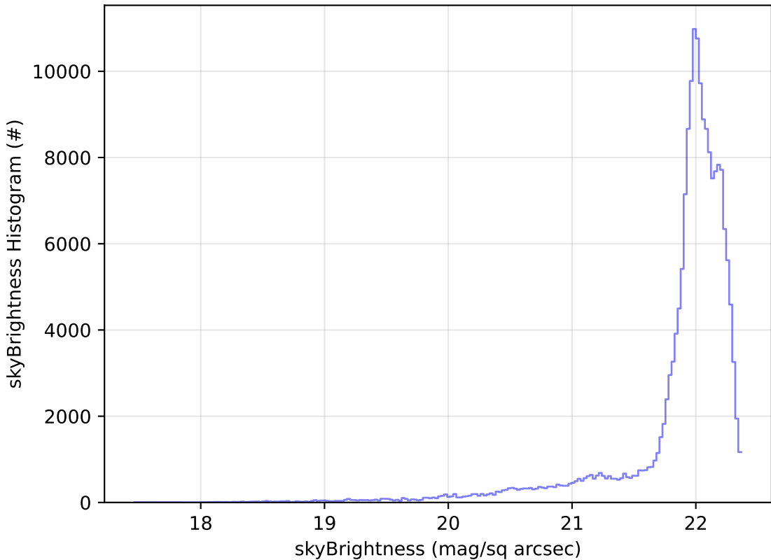
start_date_do90v3.4_10yrs All sky g band: skyBrightness Histogram
