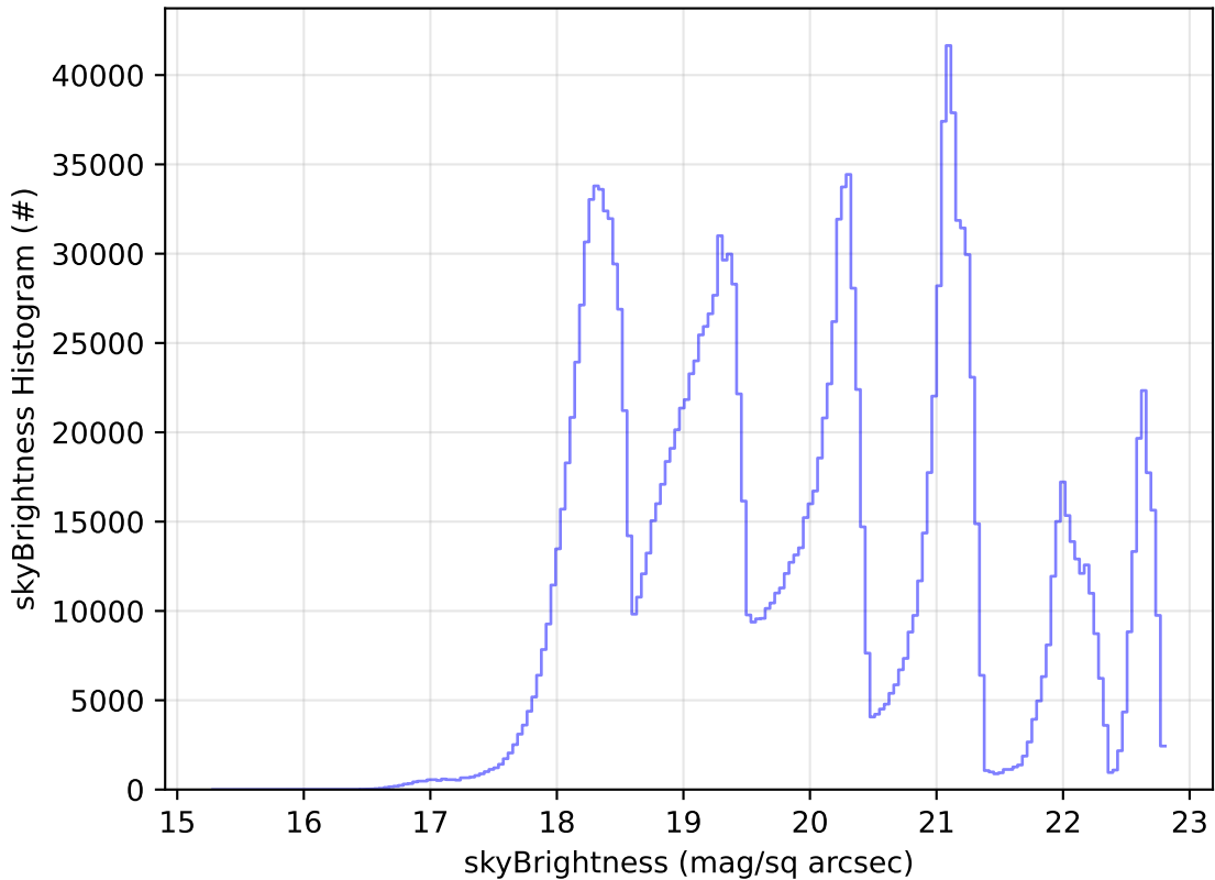
start_date_do90v3.4_10yrs All sky all bands: skyBrightness Histogram
